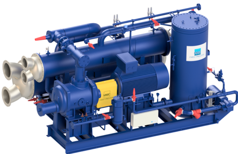
RSW unit with Howden WRV compressor
